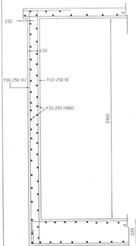
SECTION OF SIDE WALL
