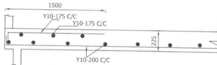
SECTION OF BOTTOM SLAB
